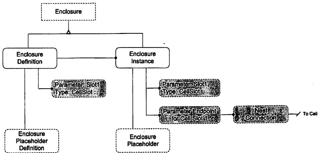
Figure 117 - Enclosure Definition Detail Model
